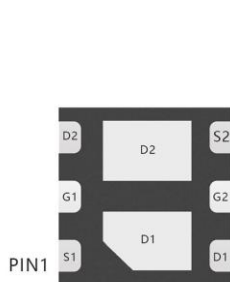
DFN2X2-6L view
