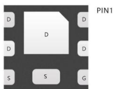
DFN2X2-6L view
