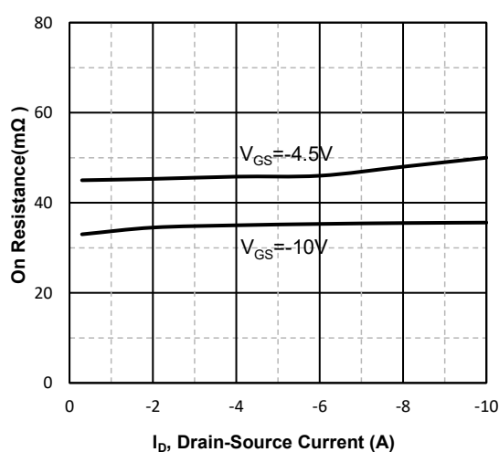
Fig4. Drain-Source on Resistance Vs. Drain-Source Current
